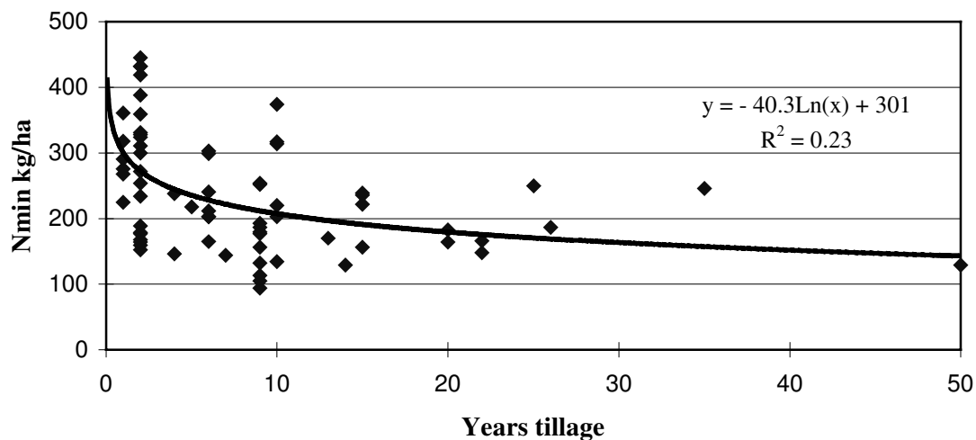
Fig. 2: Variation with number of years in tillage of Nmin in June in the 0-60 cm root profile of sugar beet.
