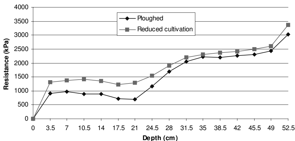
Fig. 1. Effect of cultivation treatment on cone penetration resistance at various depths
