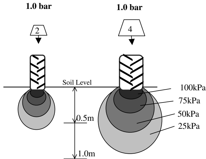
Fig. 2. Distribution of pressure stresses beneath a lightly loaded small tyre and a heavily laden large tyre exerting similar ground pressures
